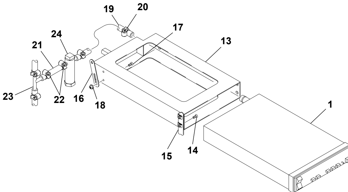
DETAIL B
