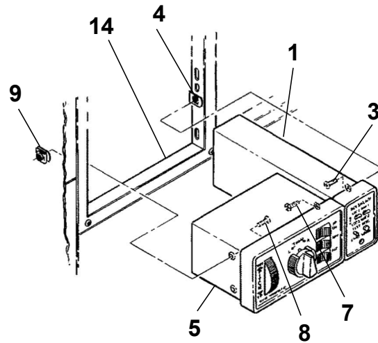
DETAIL A USED WITH AUTOPILOT
