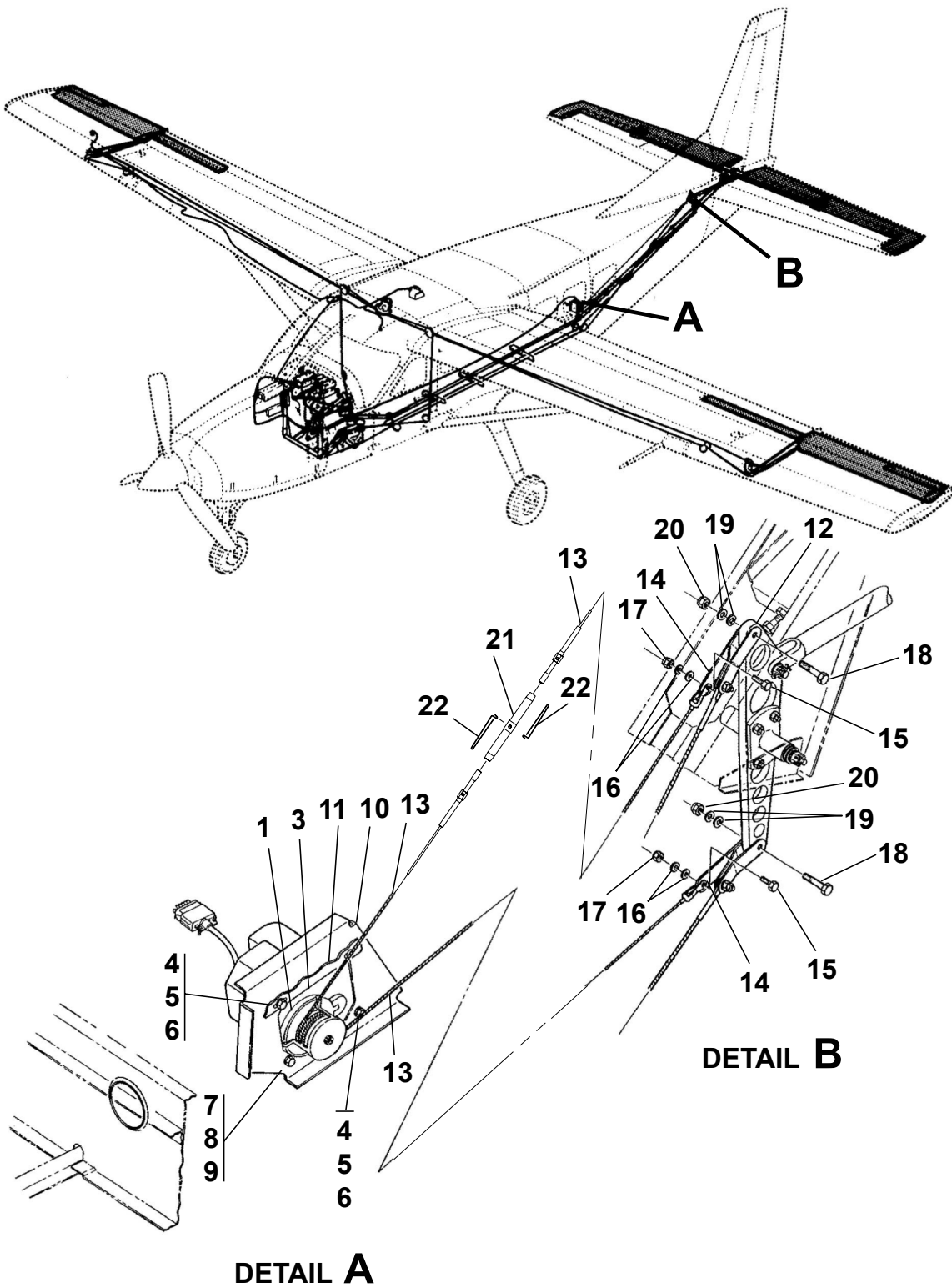
PITCH SERVO INSTALLATION - KING AUTOPILOT Figure 01. (Sheet 1)
