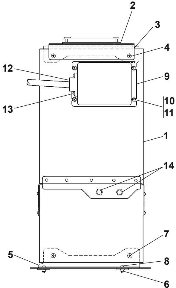
DETAIL A KAP 150 AND KFC 150
