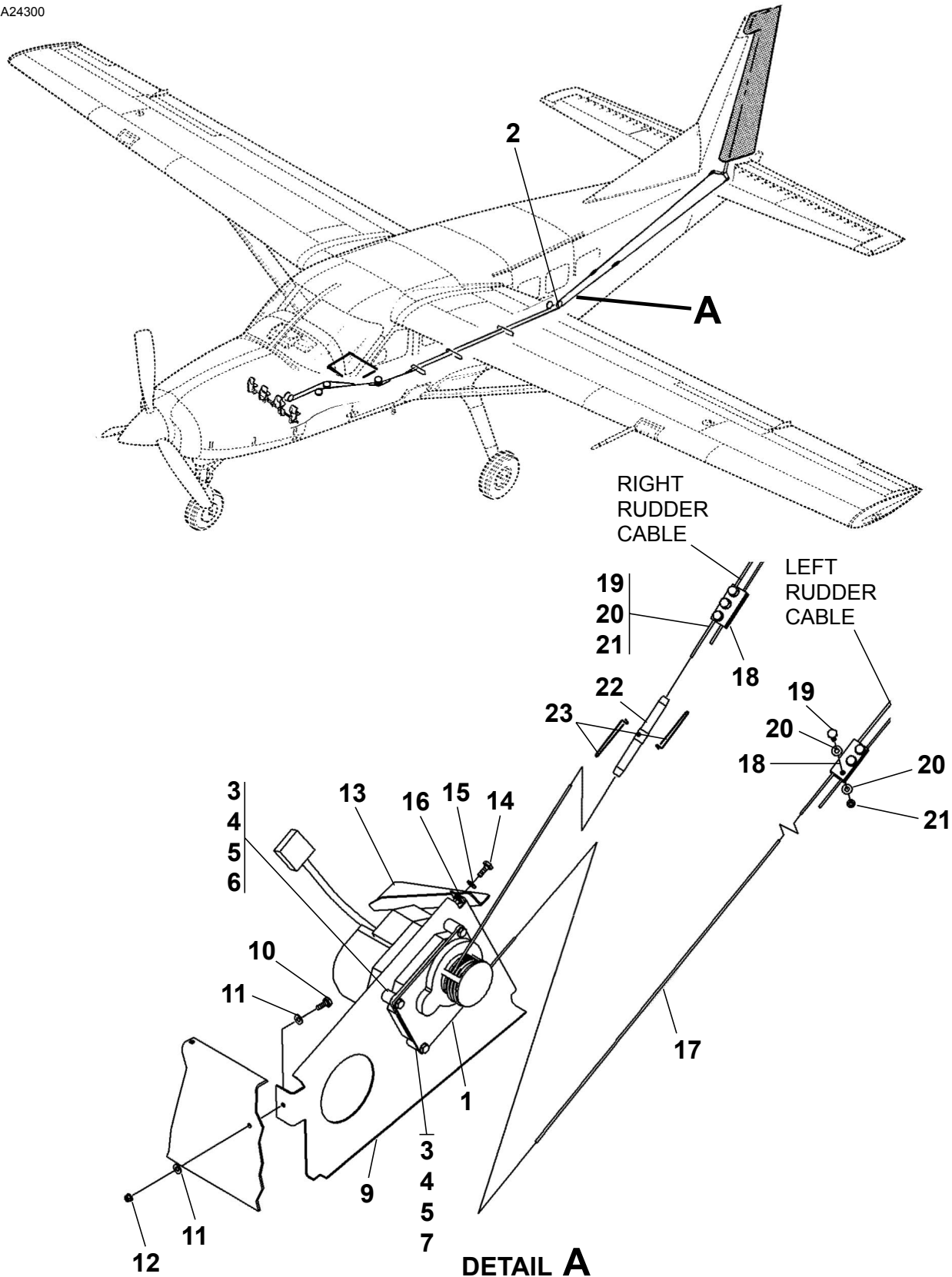
YAW DAMPER SERVO INSTALLATION Figure 01. (Sheet 1)
