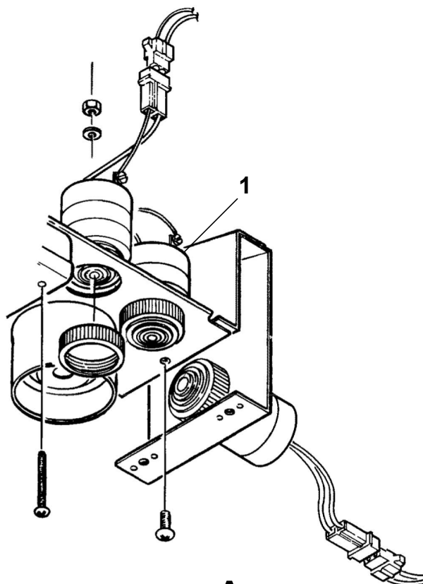
DETAIL A
