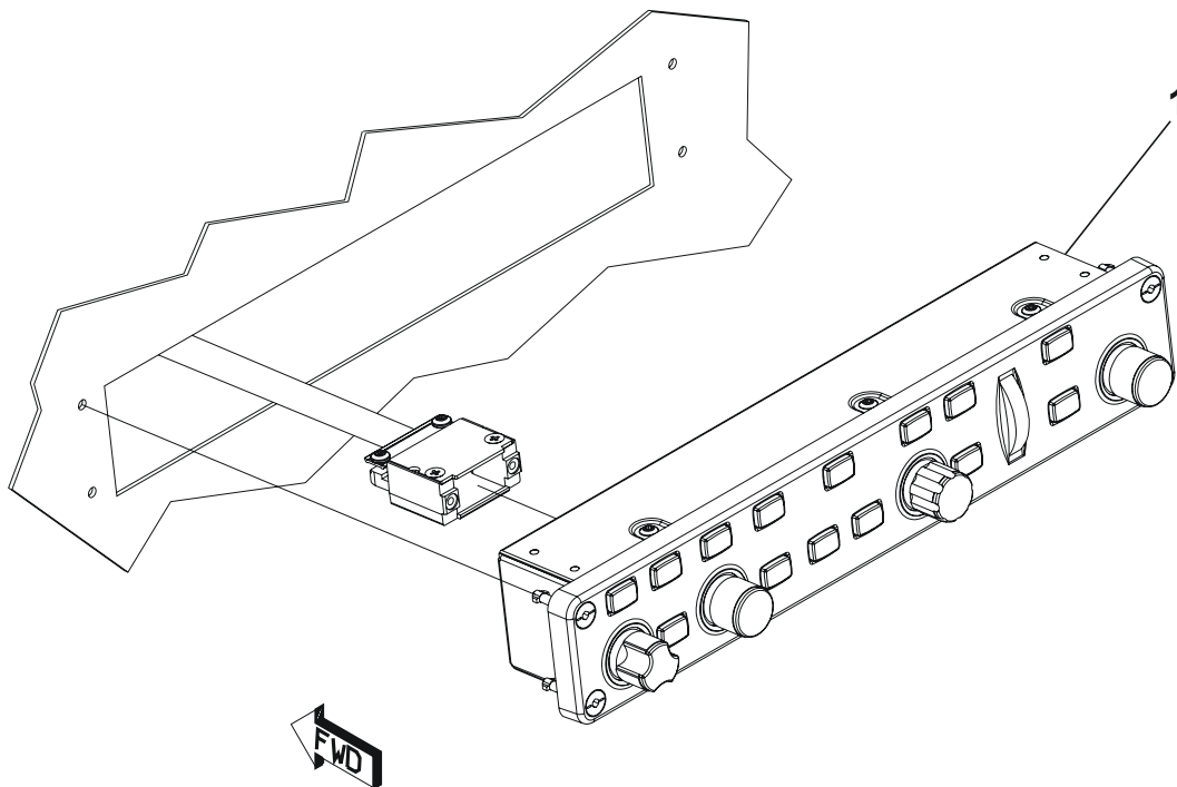
DETAIL B
