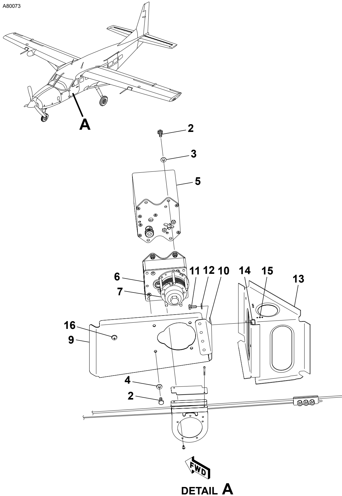
ROLL SERVO AUTOPILOT INSTALLATION Figure 01A. (Sheet 1)
